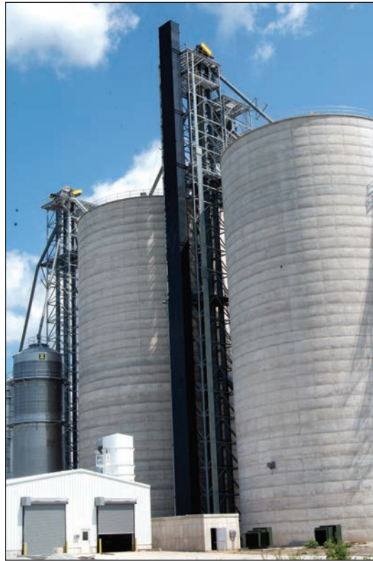
From left, dual enclosed mechanical receiving pits, two Hoffmann jumpform concrete tanks holding 500,000 bushels each, and between the tanks, two 20,000-bph Union Iron legs feeding two Union iron rotary distributors.
